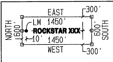
TYPICAL CLAIM DETAIL (NOT TO SCALE)
